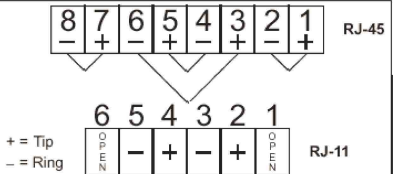
Figure 3 Plug Polarities
