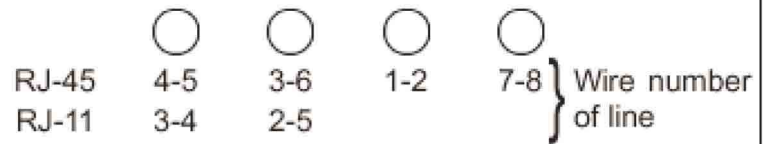
Figure 1 Wiring Schemes
